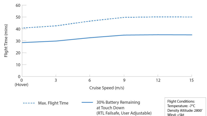
SwitchBlade-Elite 2.3 | Flight Time v Cruise Speed 0.5 kg payload (α6400 or RX1Rii nadir-mounted)
